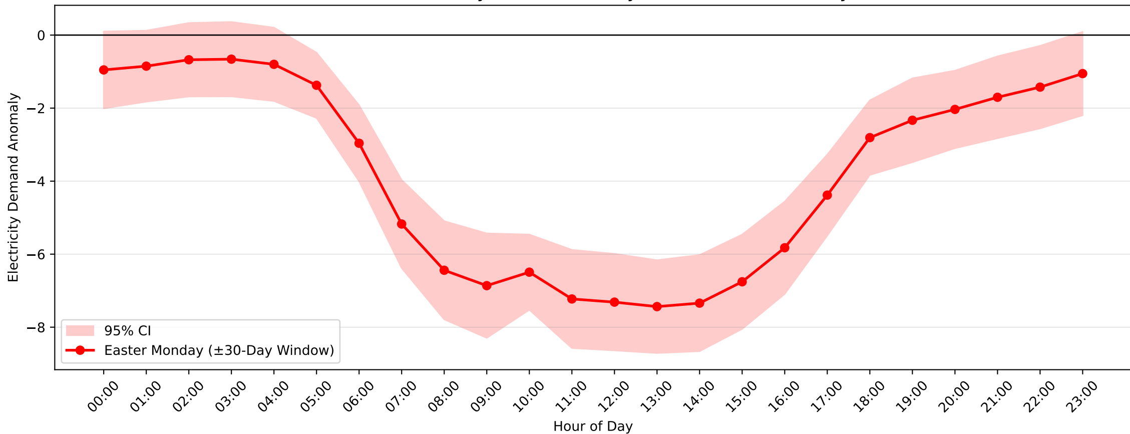
Mascot Demand Anomaly: Easter Monday (2004-2017, \pm 30 -Day Window)
